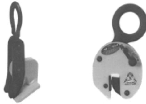
Examples of types of plate clamps
